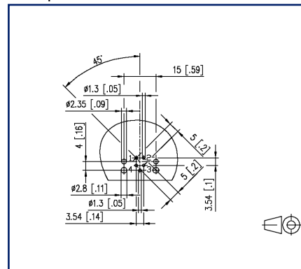
Drill pattern
