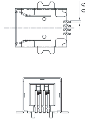
PC Board Layout - Component Side
