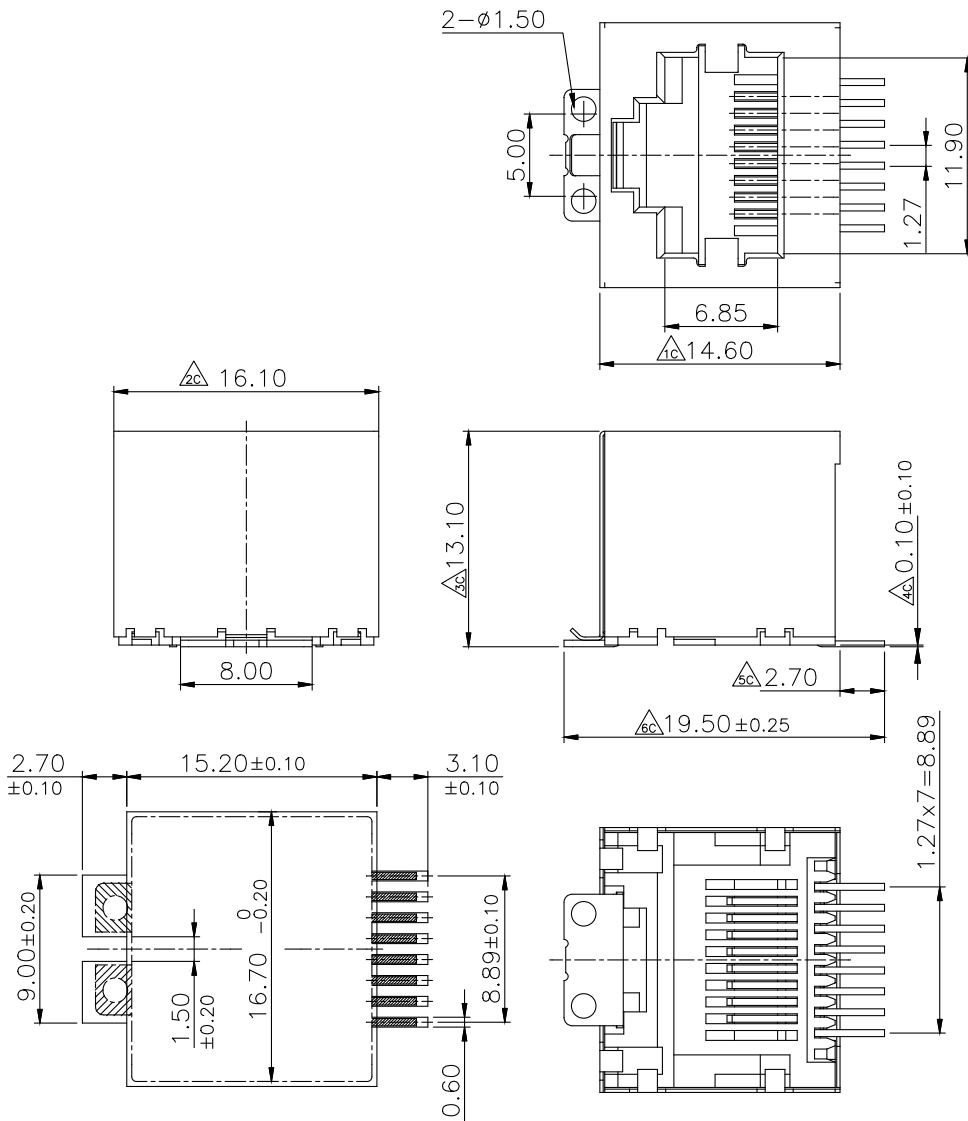
PCB LAYOUT/TOP VIEW
