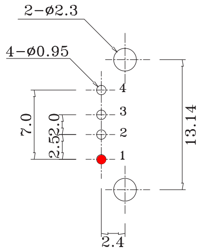
PC Board Layout - Bottom View
