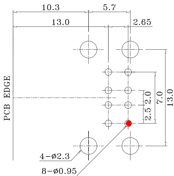
PC Board Layout - Bottom View
