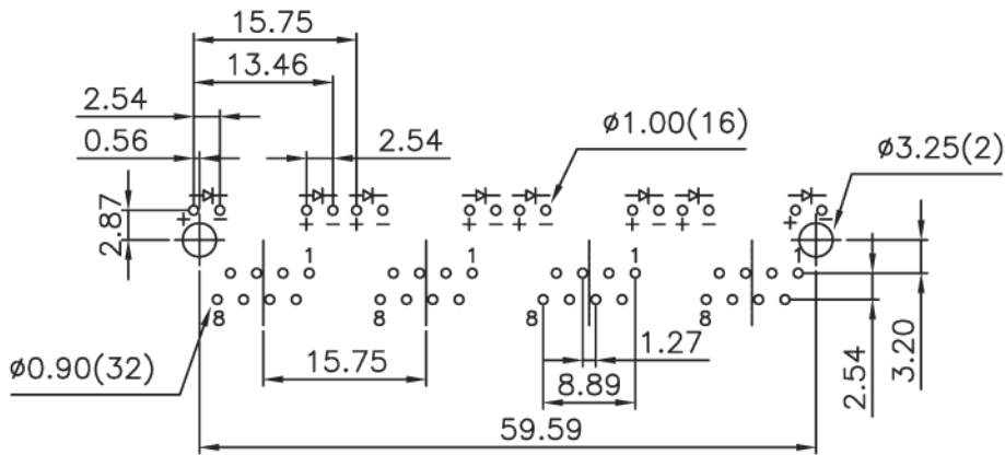
PCB LAYOUT
