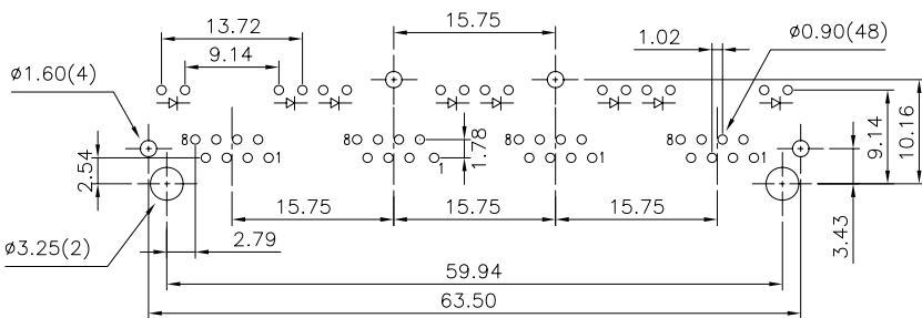
PCB LAYOUT (Ref.)
