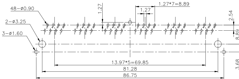
PCB LAYOUT/TOP VIEW
