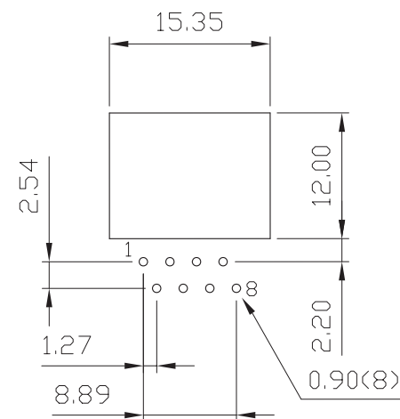
PCB LAYOUT Ref.
