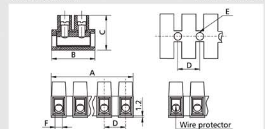
Dimensions in mm 1 mm = 0.0394 in.
