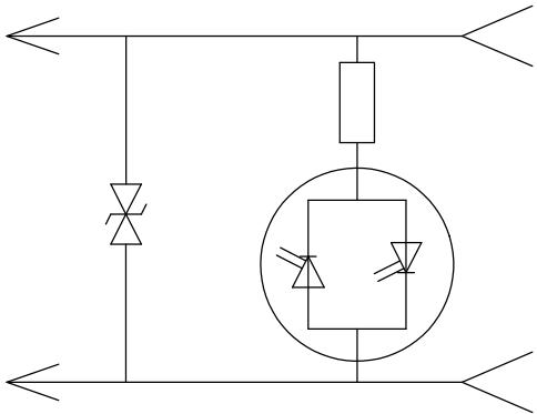
LED W/ DUAL ZENOR DIODES
