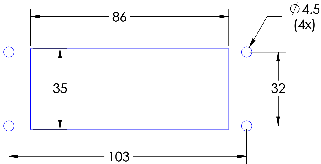
PANEL CUTOUT
