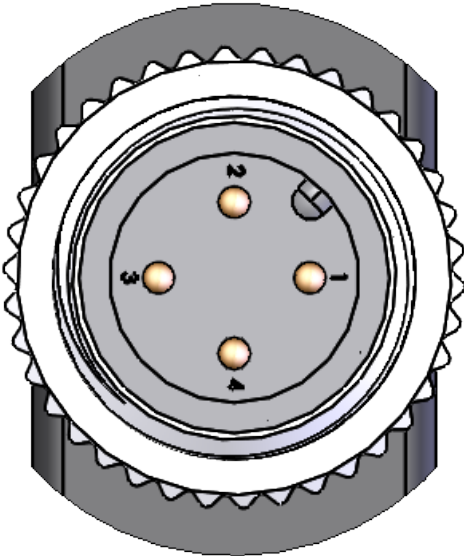
DETAIL B SCALE 4 : 1
