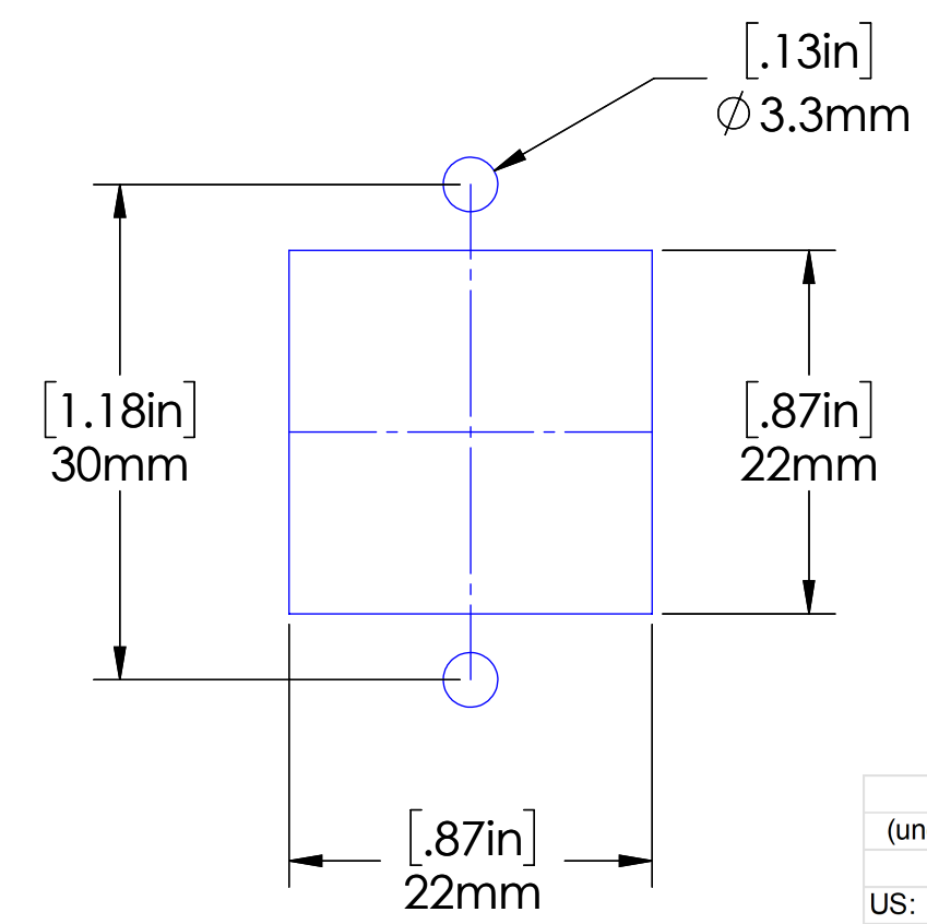
PANEL CUTOUT
