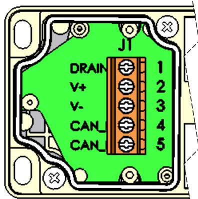
WIRING CHAMBER
