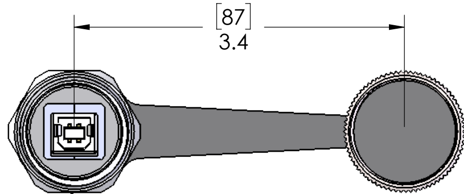
USB TYPE B FEMALE
