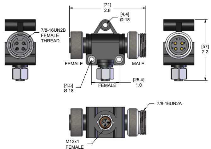
7/8"-16UN to M12 "T" Connector
