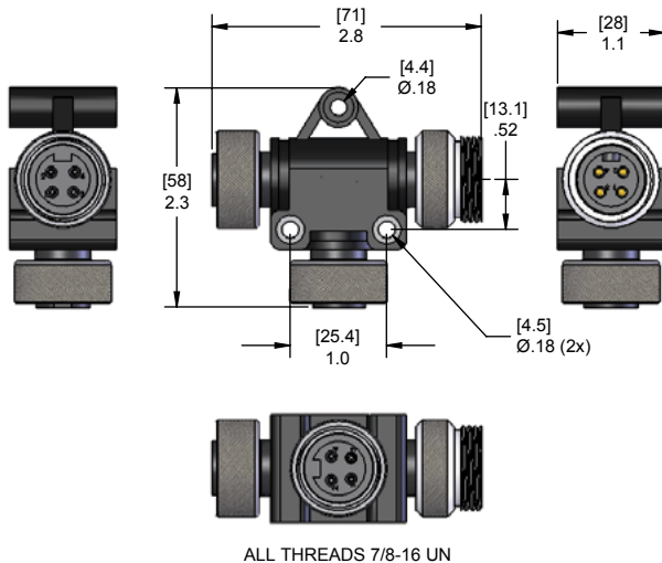
7/8"-16UN to 7/8"-16UN "T" Connector
