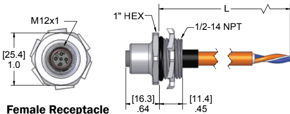
Female Receptacle
