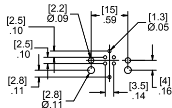
5 Pole Male Right Angle Layout
