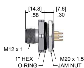
Male Receptacles
