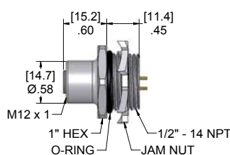
Female Receptacles
