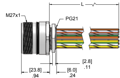
PG21 Threads
