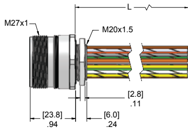
M20 Threads
