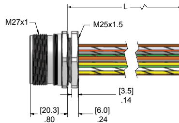
M25 Threads
