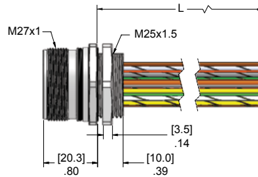
M25L Threads
