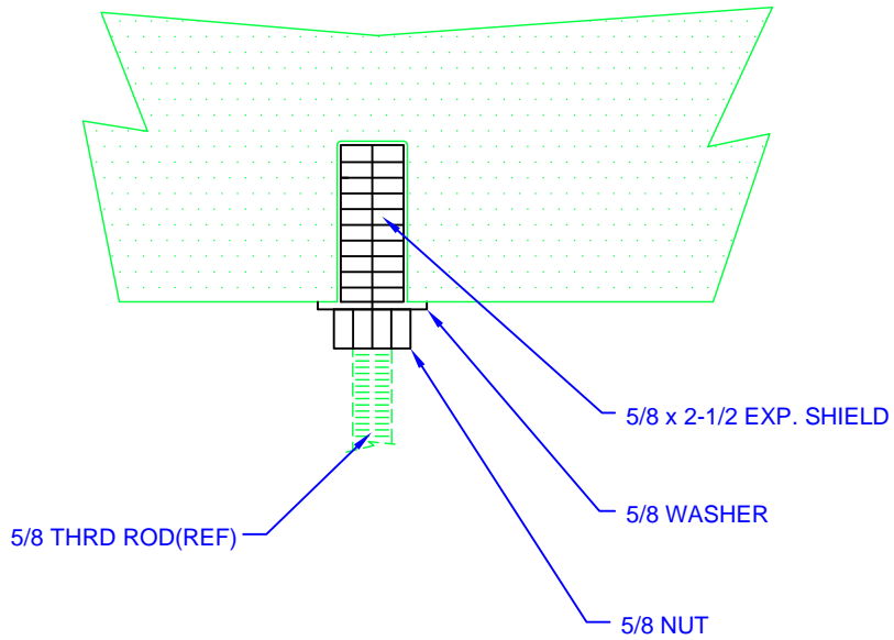
ROD CEILING ANCHOR SHIELD IN CONCRETE
