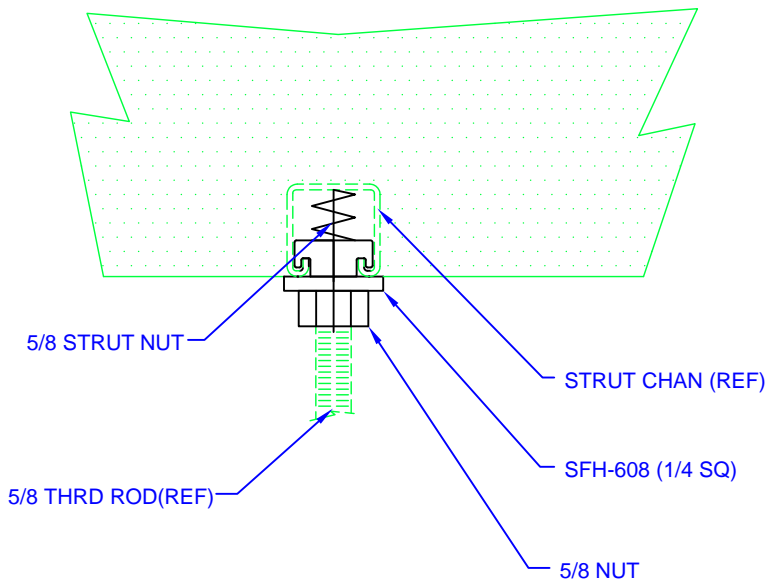
ROD CEILING ANCHOR INTO EMBEDDED CHANNEL PER GR-1275
